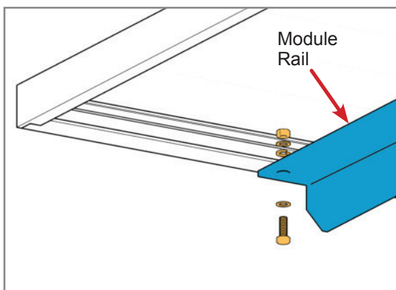
Secure Modules at each of their four attachment points with 1/4" x 3/4" Bolt, two Flat Washers, Lock Washer, and Nut.
