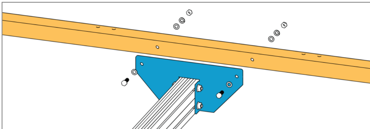
Secure Module Rails to Rail Brackets with 3/8" x 1" Bolt, two Flat Washers, Lock Washer and Nut.
