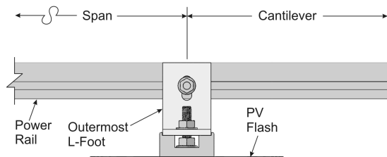
Figure 5-1: Cantilever Measurement
