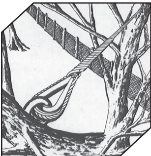
TREE-GRIP Dead-end showing THIMBLE-LOOP insert
