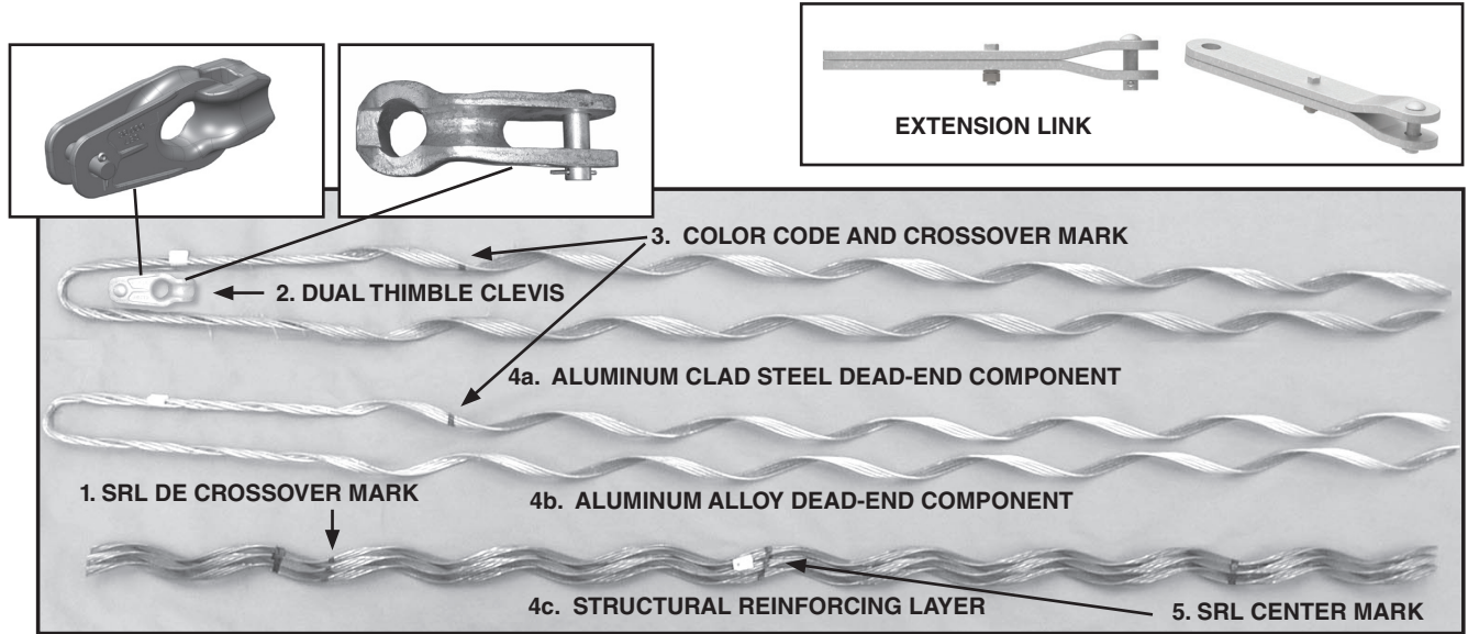
THERMOLIGN DEAD-END AND ASSOCIATED HARDWARE
