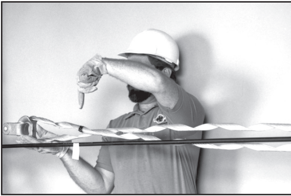
Positioning the THERMOLIGN DEAD-END
