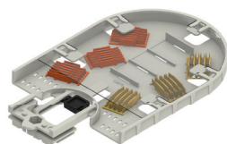
Thin Profile Short Flip Tray – 36 CT. Single Fusion or 144 CT. Mass Fusion Catalog Number: 80814403
