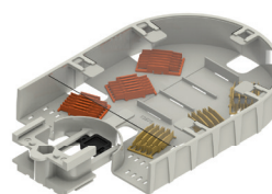
Deep Profile Short Flip Tray – 36 CT. Single Fusion or 144 CT. Mass Fusion Catalog Number: 80814404
