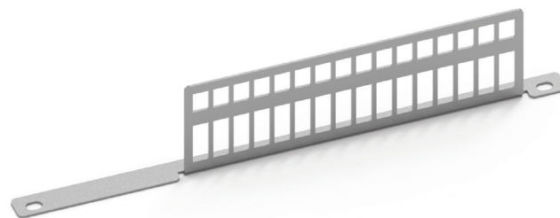
COYOTE Short 32-Position Bulkhead Bracket Included with Catalog Number: CXD622U-003
