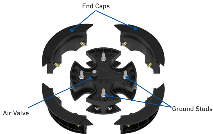
6.5" Dome Closure Patented Segmented End Plate
