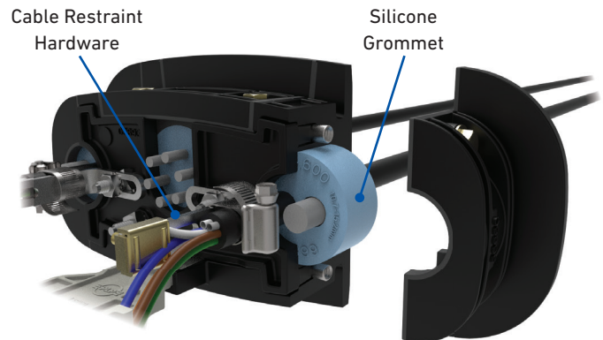
COYOTE ONE Dome End Plate Cap – Exploded View
