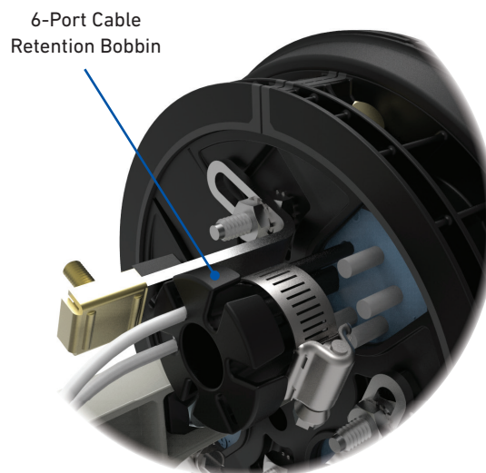
Installed 6-Port Cable Retention Bobbin for 6-Hole Grommet
