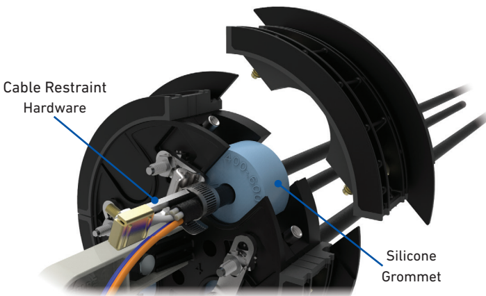
6.5" Dome End Plate Cap – Exploded View
