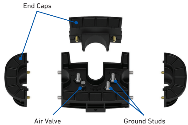
COYOTE® ONE Dome Closure Patented Segmented End Plate
