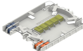
Catalog Number: 80808945 Short – Deep Profile Single Fusion/Double Stack 40 Splice Count
