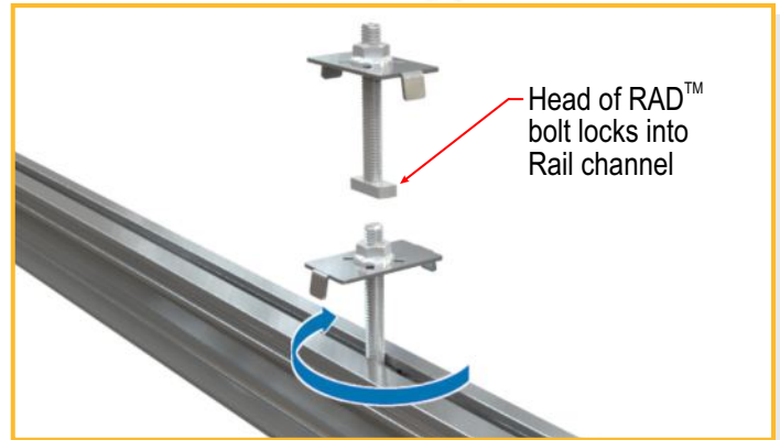
RAD Hardware: Patented drop and twist design locks bolt into rail for quick and easy top down mid-clamp installation.
