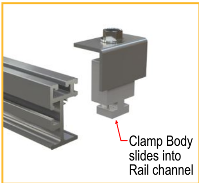
Universal End Clamp: Fits wide range of modules and all Power Rail profiles.
