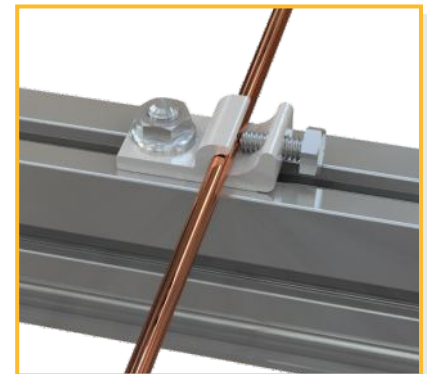
Grounding Lug: Use one for each row of modules.
