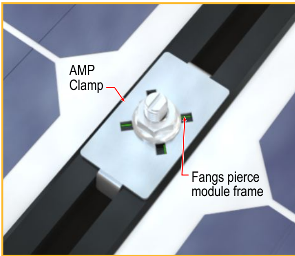
AMP Clamp: Self grounding mid-clamp penetrates anodized module frame, effectively bonding modules to rails.
