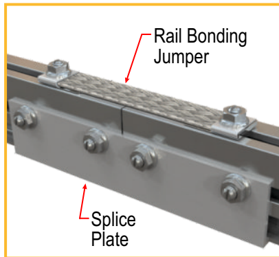
Rail Bonding Jumper: Bonds rail-to-rail splices. Only used on rail with Grounding Lug.
