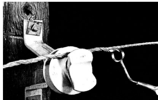
SIDE TIE
