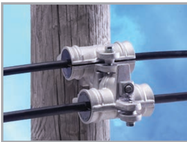
ADSS Supports
