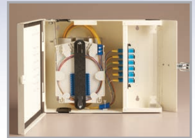
Fiber Distribution Cabinets
