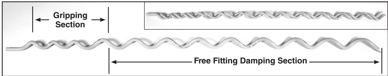
Spiral Vibration Damper or Dielectric Damper as received at job site.
