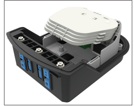
Splice + Adapters
