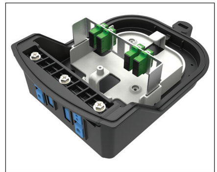
Adapter Organizer
