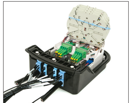
Splice + Adapters
