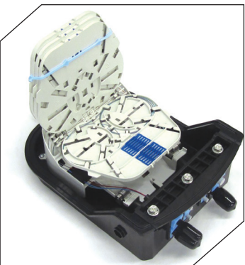
Splice Organizer
